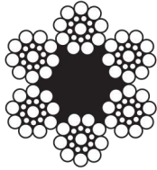
8x19 Seale Fiber Core ( 8 x 9/9/1 )
