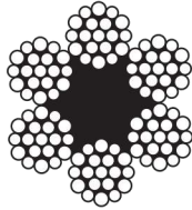
8x19 Warrington Fiber Core ( 8 x 6 & 6/6/1 )
